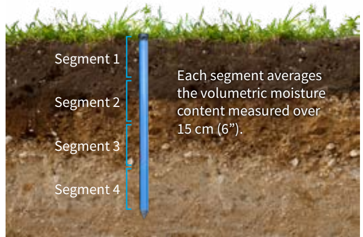
The Stevens GroPoint Profile is ideal for measuring water movement across multiple soil horizons.
